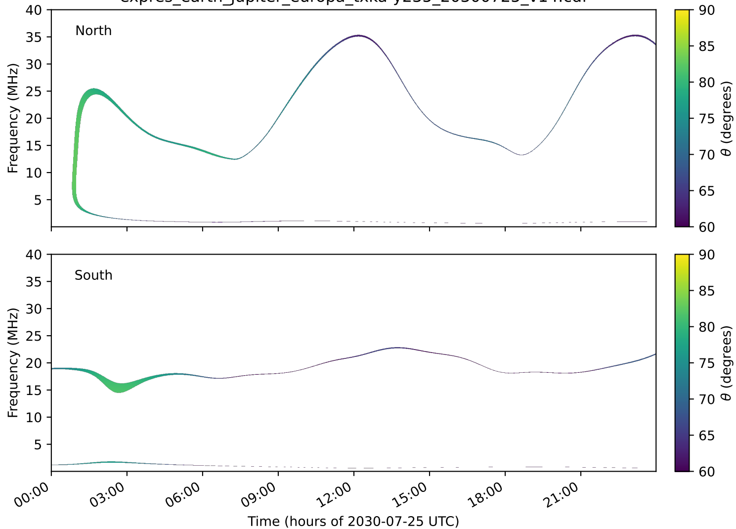
expres_earth_jupiter_europa_txka-y235_20300725_v14.cdf
