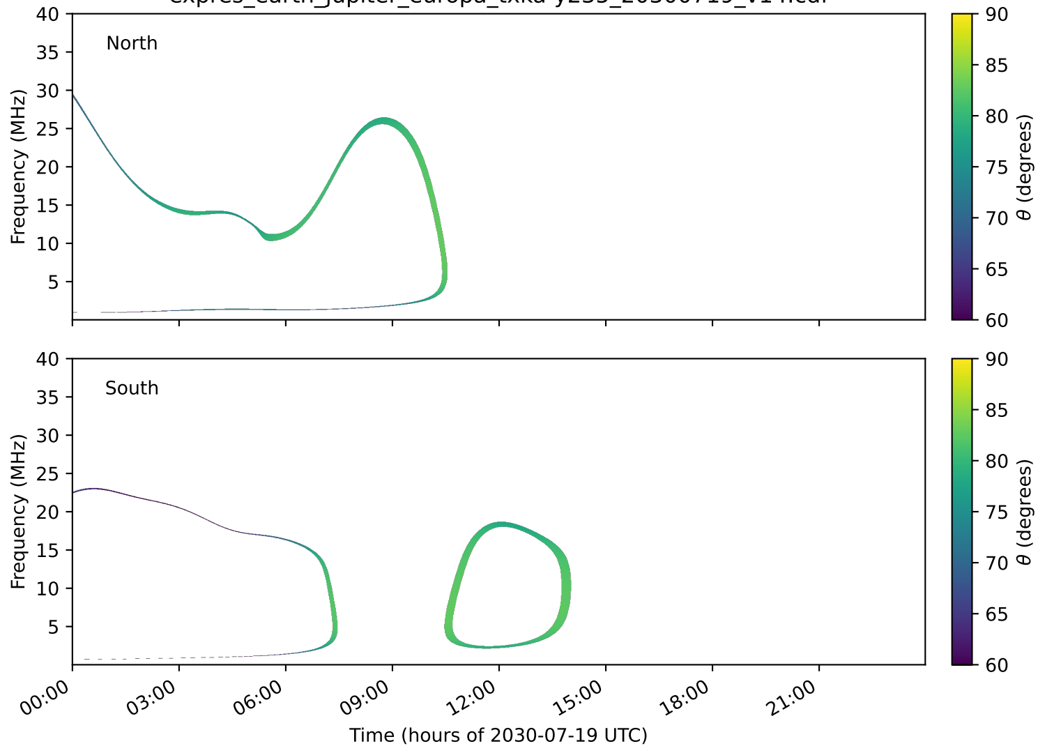
expres_earth_jupiter_europa_txka-y235_20300719_v14.cdf
