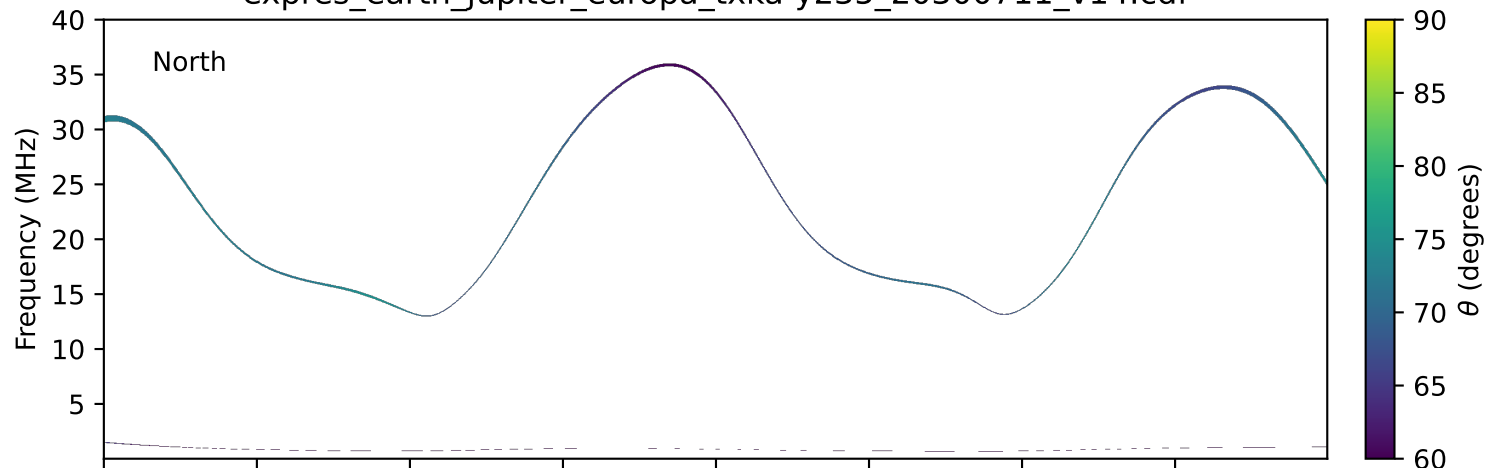
expres_earth_jupiter_europa_txka-y235_20300711_v14.cdf
