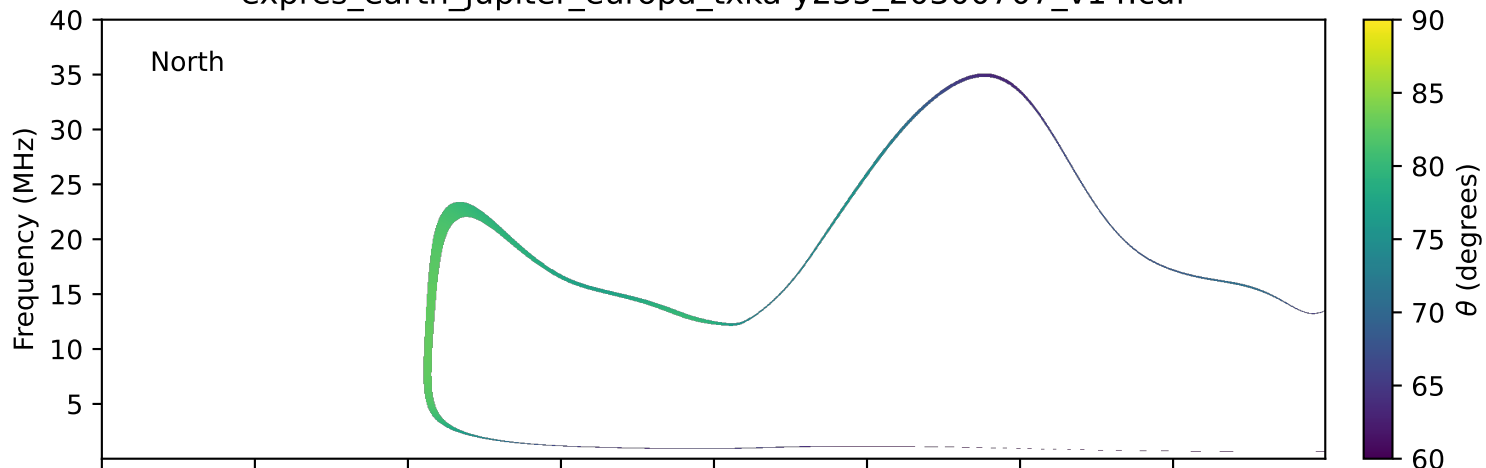
expres_earth_jupiter_europa_txka-y235_20300707_v14.cdf
