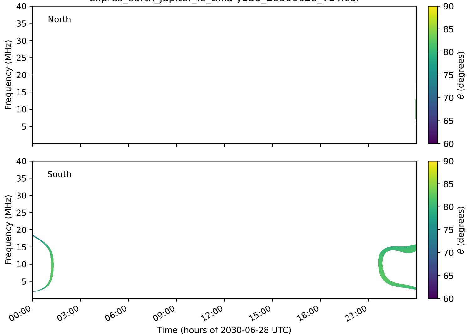
expres_earth_jupiter_io_txka-y235_20300628_v14.cdf
