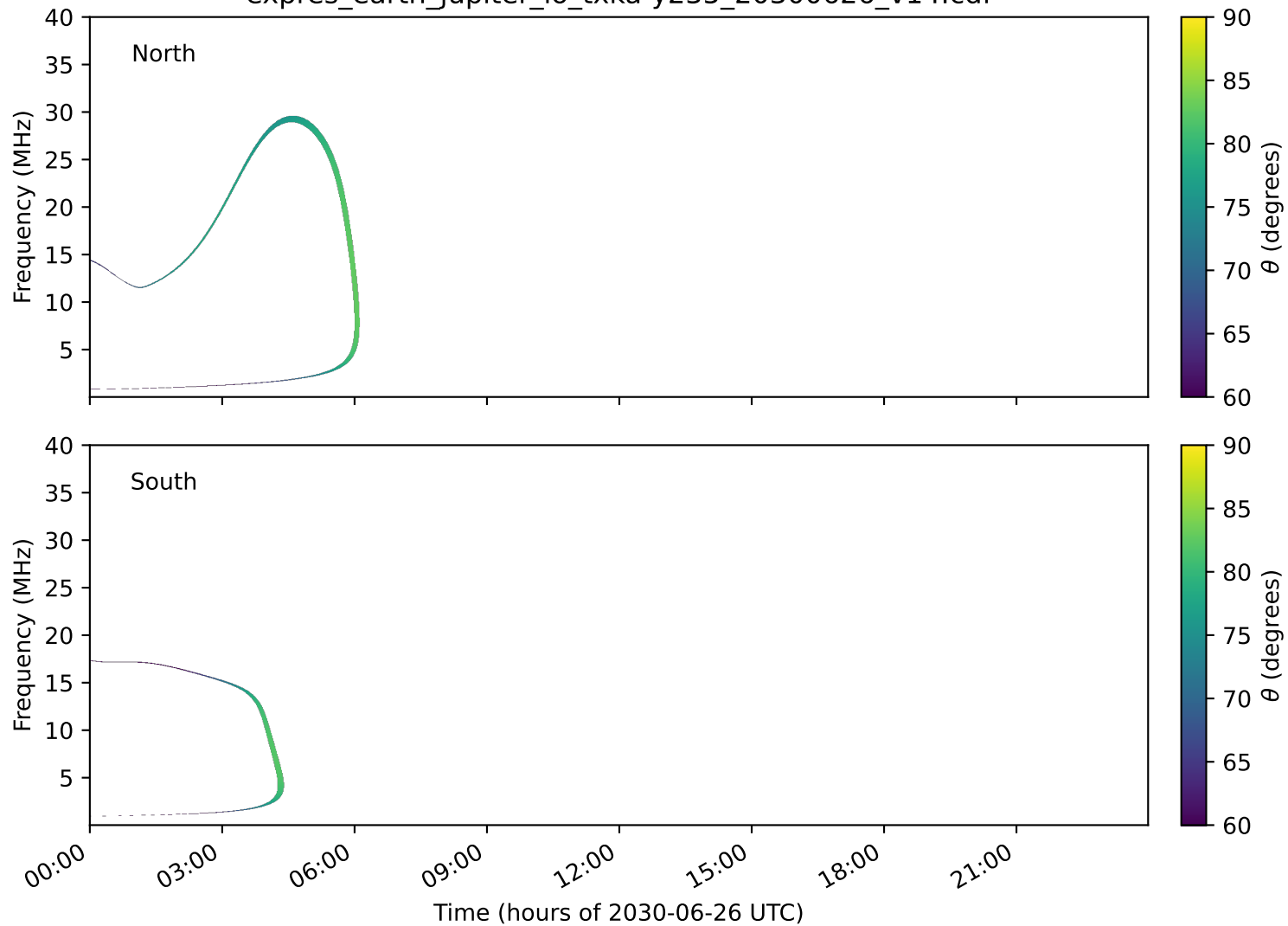
expres_earth_jupiter_io_txka-y235_20300626_v14.cdf
