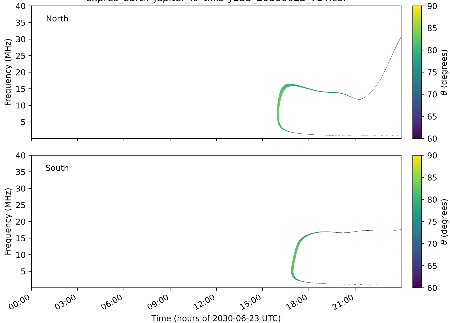
expres_earth_jupiter_io_txka-y235_20300623_v14.cdf
