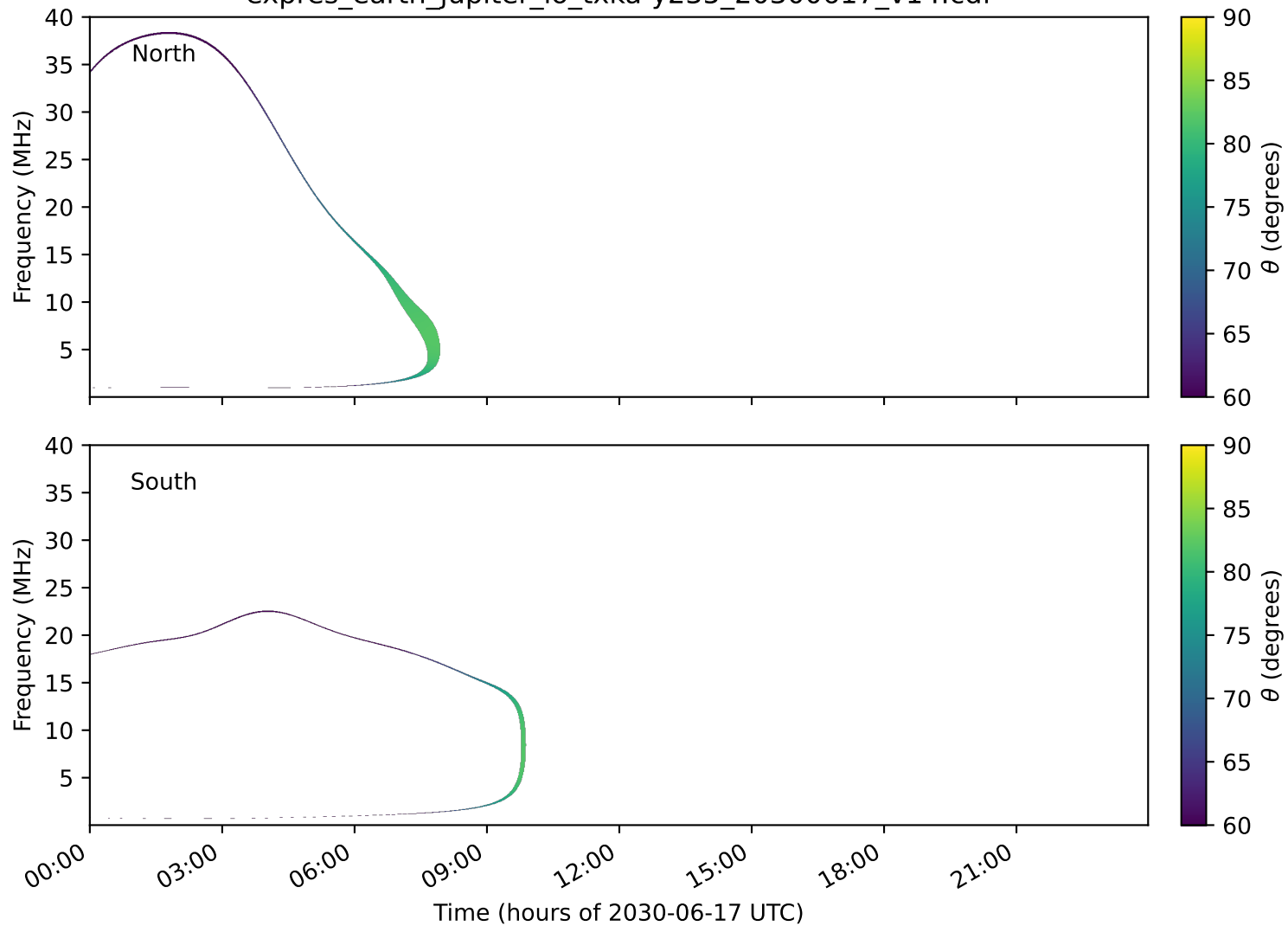
expres_earth_jupiter_io_txka-y235_20300617_v14.cdf
