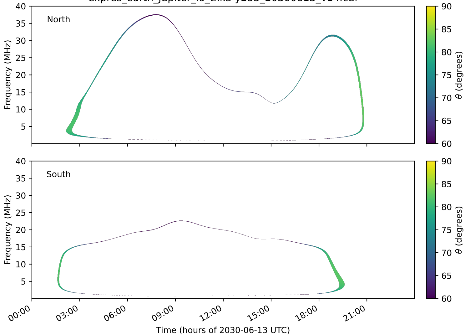
expres_earth_jupiter_io_txka-y235_20300613_v14.cdf
