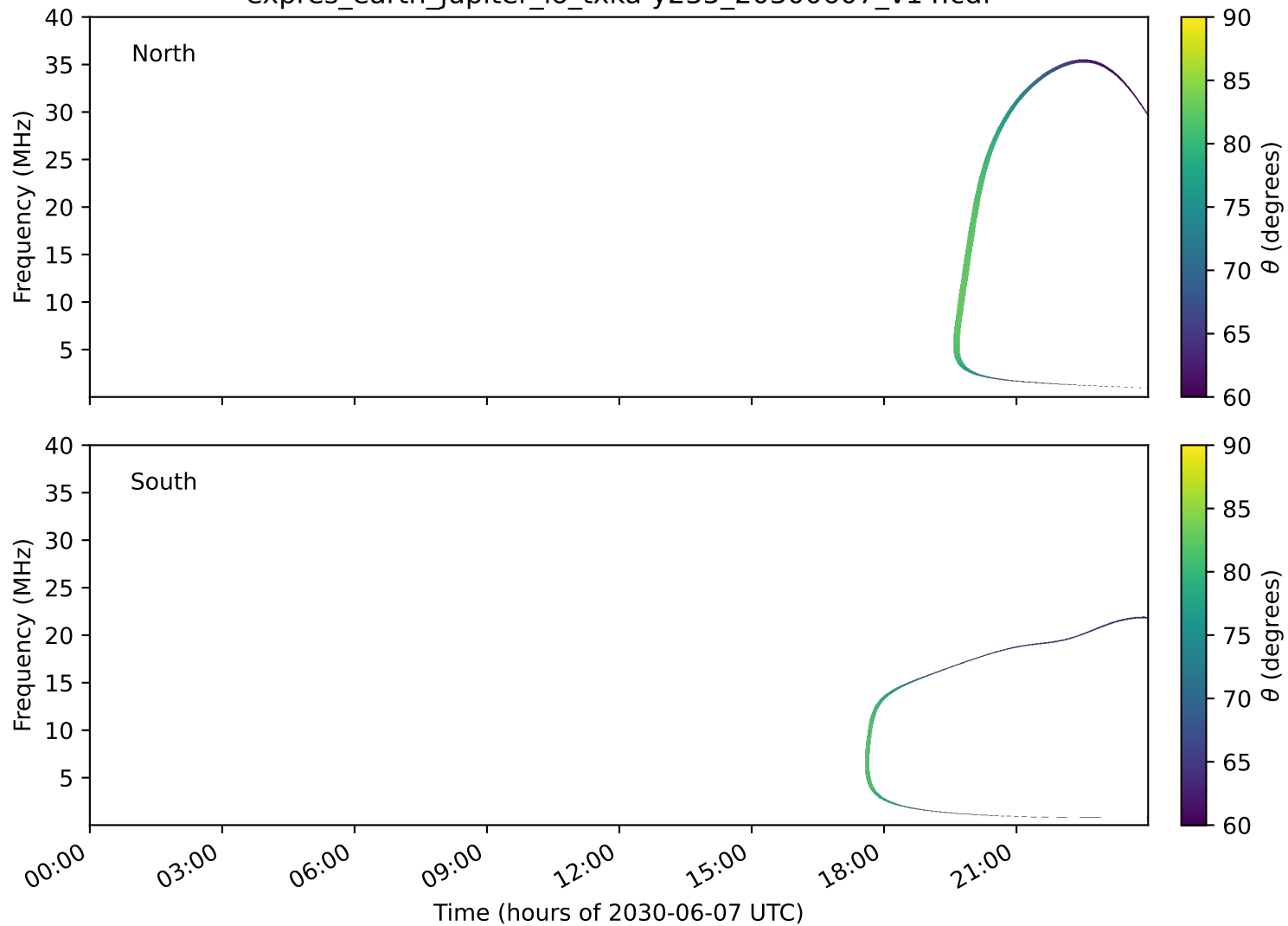
expres_earth_jupiter_io_txka-y235_20300607_v14.cdf
