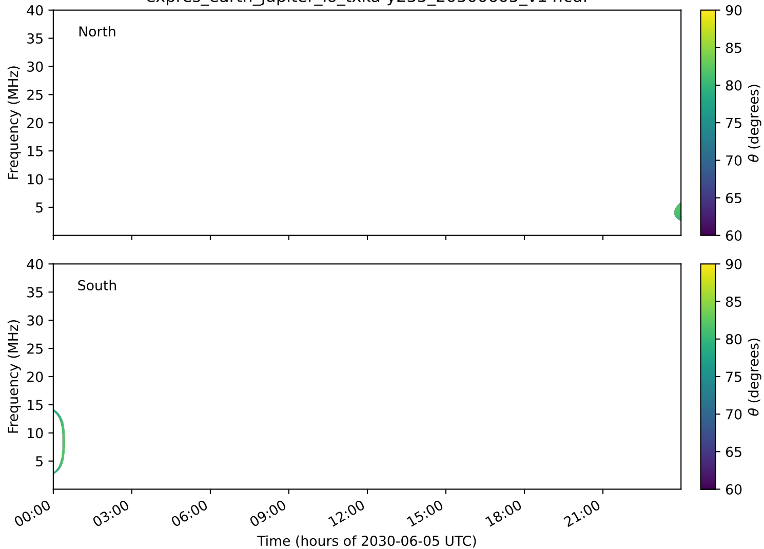
expres_earth_jupiter_io_txka-y235_20300605_v14.cdf
