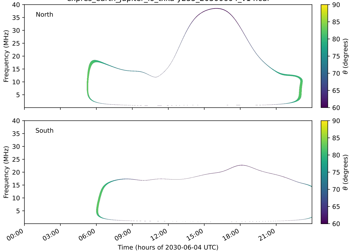
expres_earth_jupiter_io_txka-y235_20300604_v14.cdf
