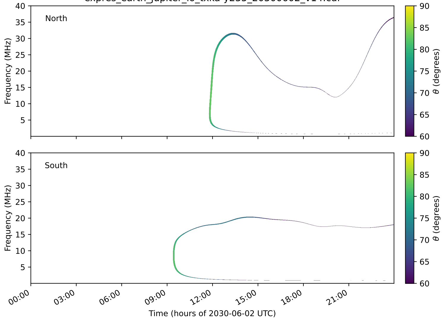
expres_earth_jupiter_io_txka-y235_20300602_v14.cdf
