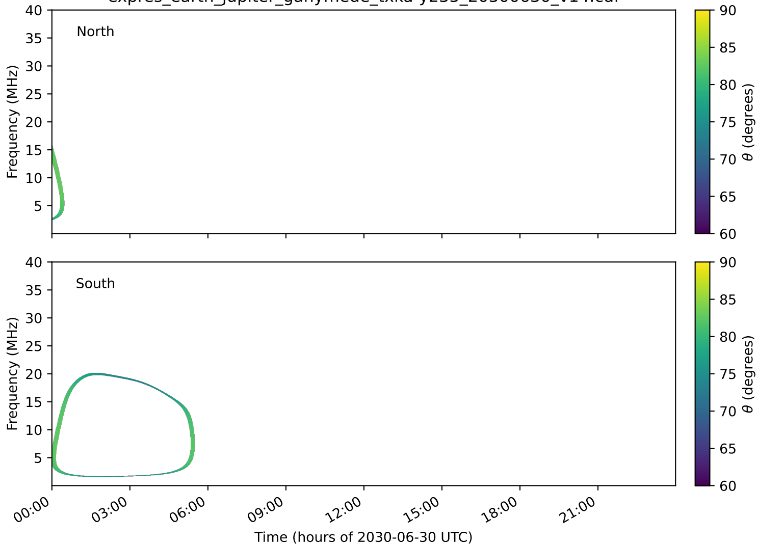
expres_earth_jupiter_ganymede_txka-y235_20300630_v14.cdf
