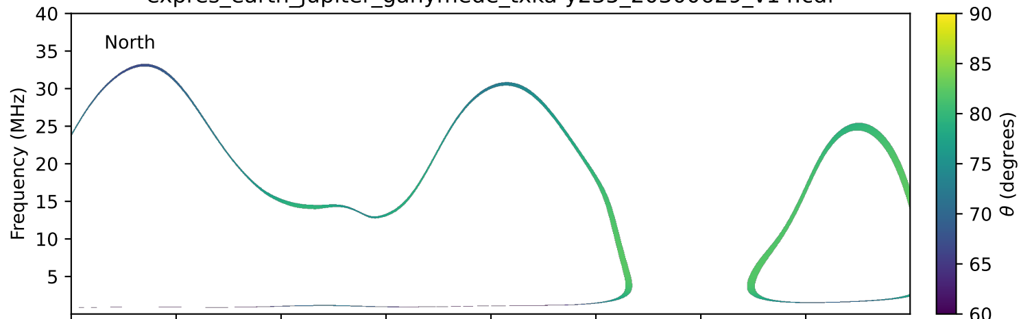
expres_earth_jupiter_ganymede_txka-y235_20300629_v14.cdf
