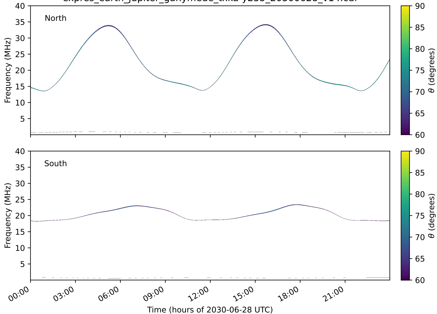
expres_earth_jupiter_ganymede_txka-y235_20300628_v14.cdf
