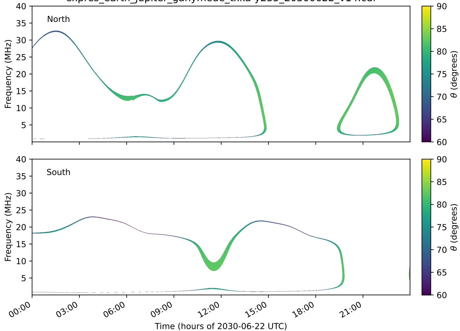
expres_earth_jupiter_ganymede_txka-y235_20300622_v14.cdf
