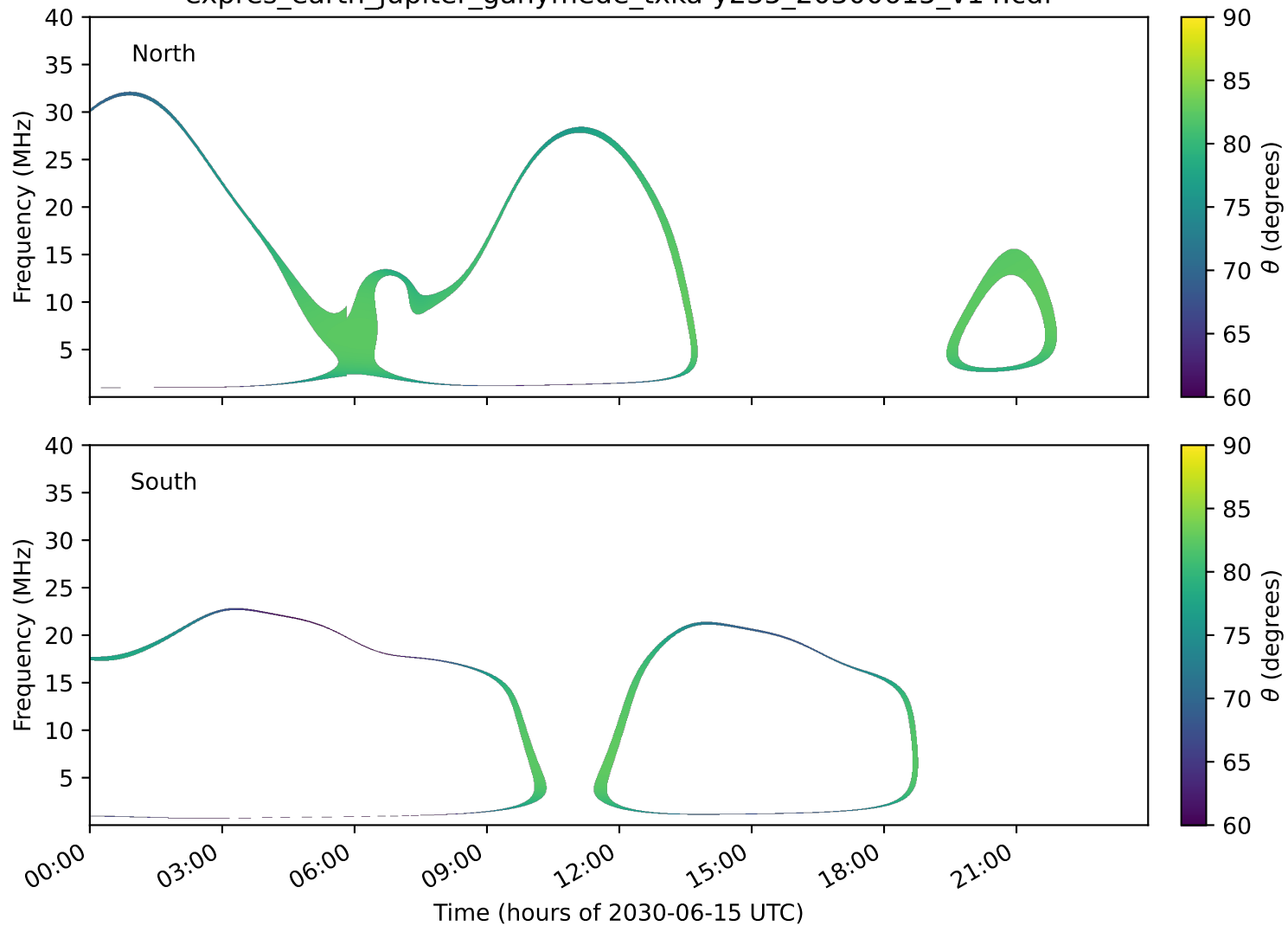
expres_earth_jupiter_ganymede_txka-y235_20300615_v14.cdf
