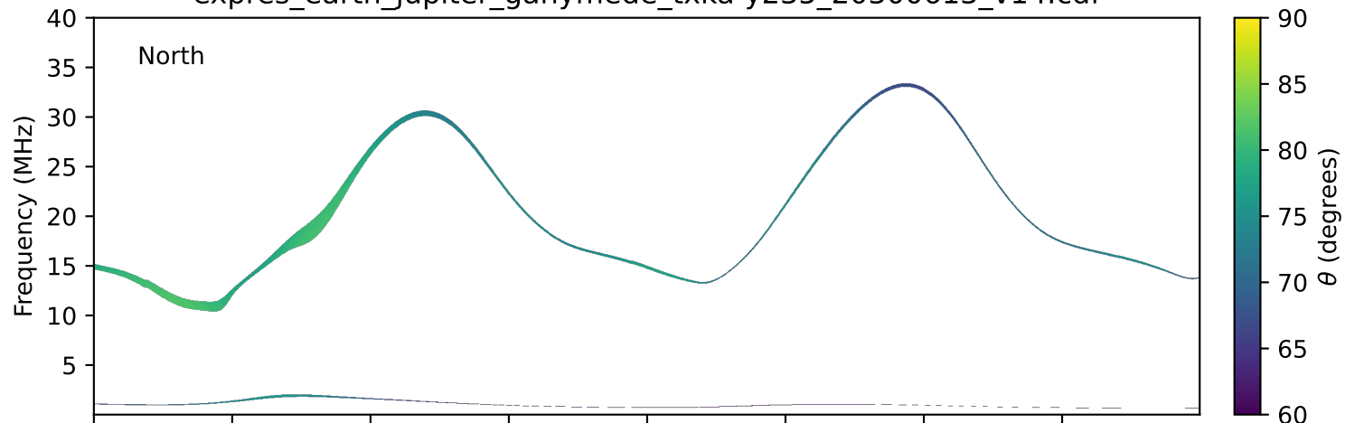
expres_earth_jupiter_ganymede_txka-y235_20300613_v14.cdf
