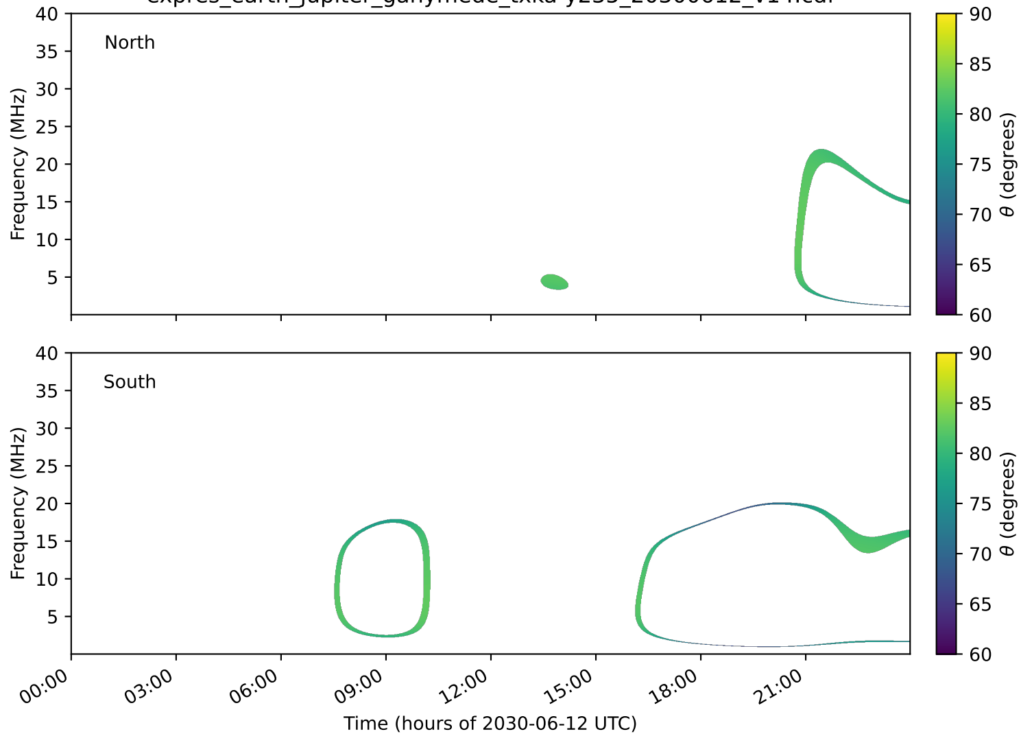
expres_earth_jupiter_ganymede_txka-y235_20300612_v14.cdf
