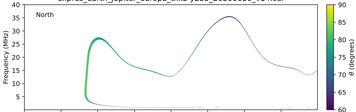
expres_earth_jupiter_europa_txka-y235_20300630_v14.cdf
