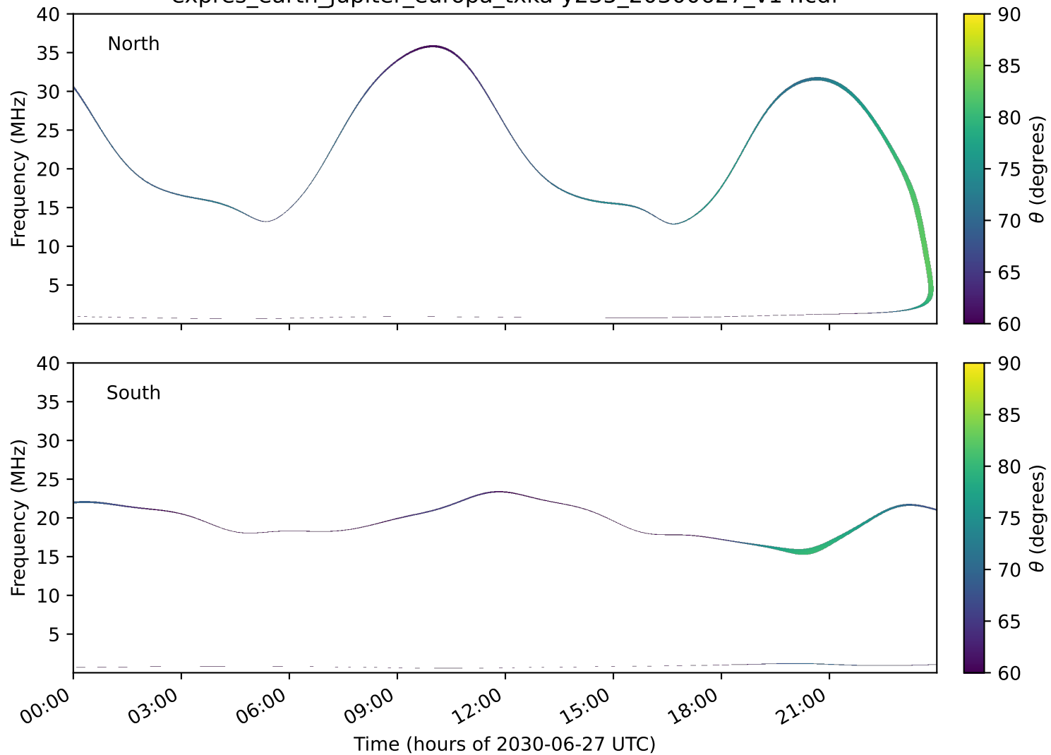
expres_earth_jupiter_europa_txka-y235_20300627_v14.cdf
