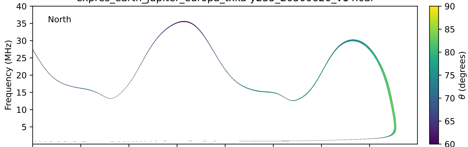
expres_earth_jupiter_europa_txka-y235_20300620_v14.cdf
