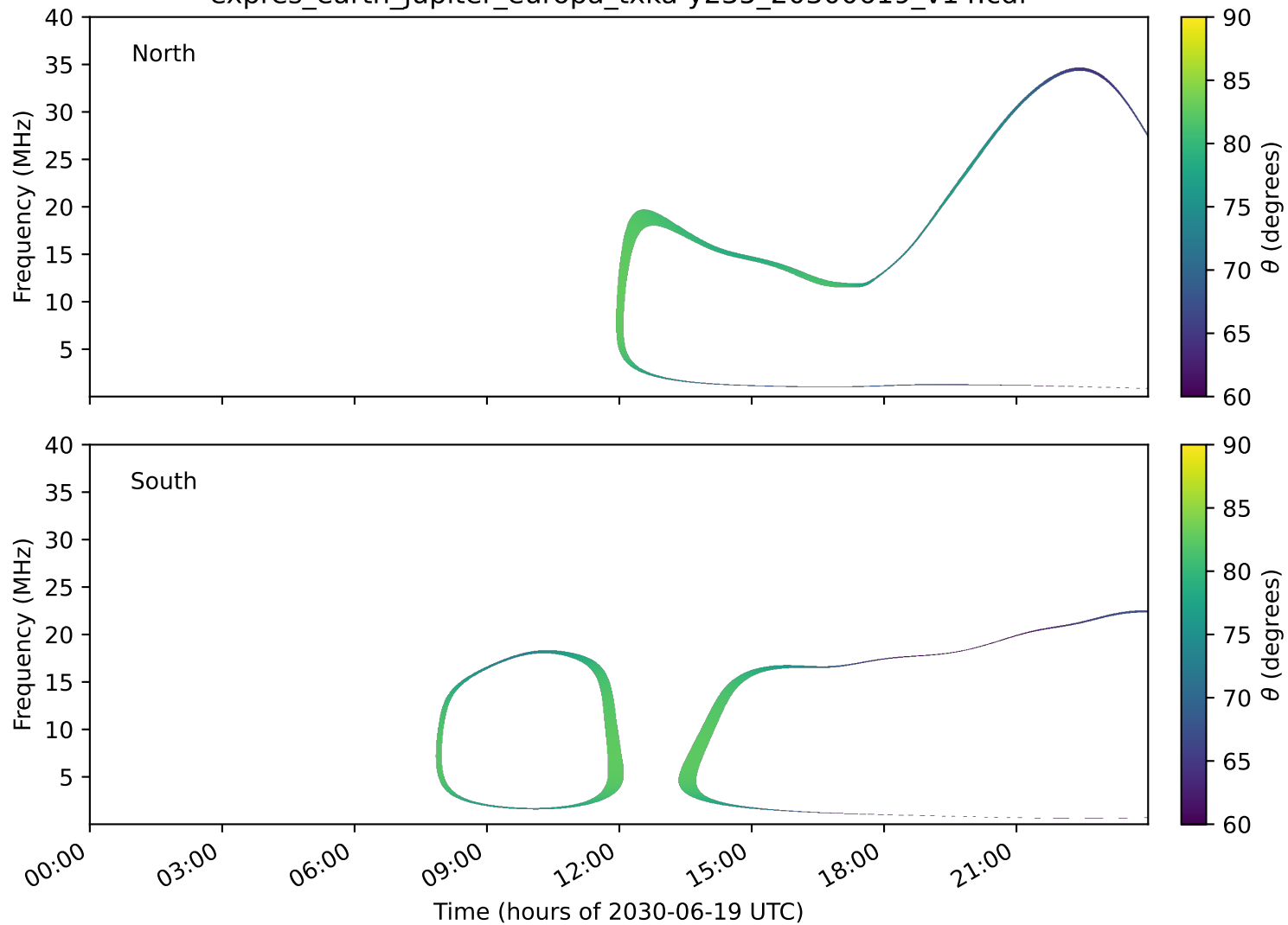
expres_earth_jupiter_europa_txka-y235_20300619_v14.cdf
