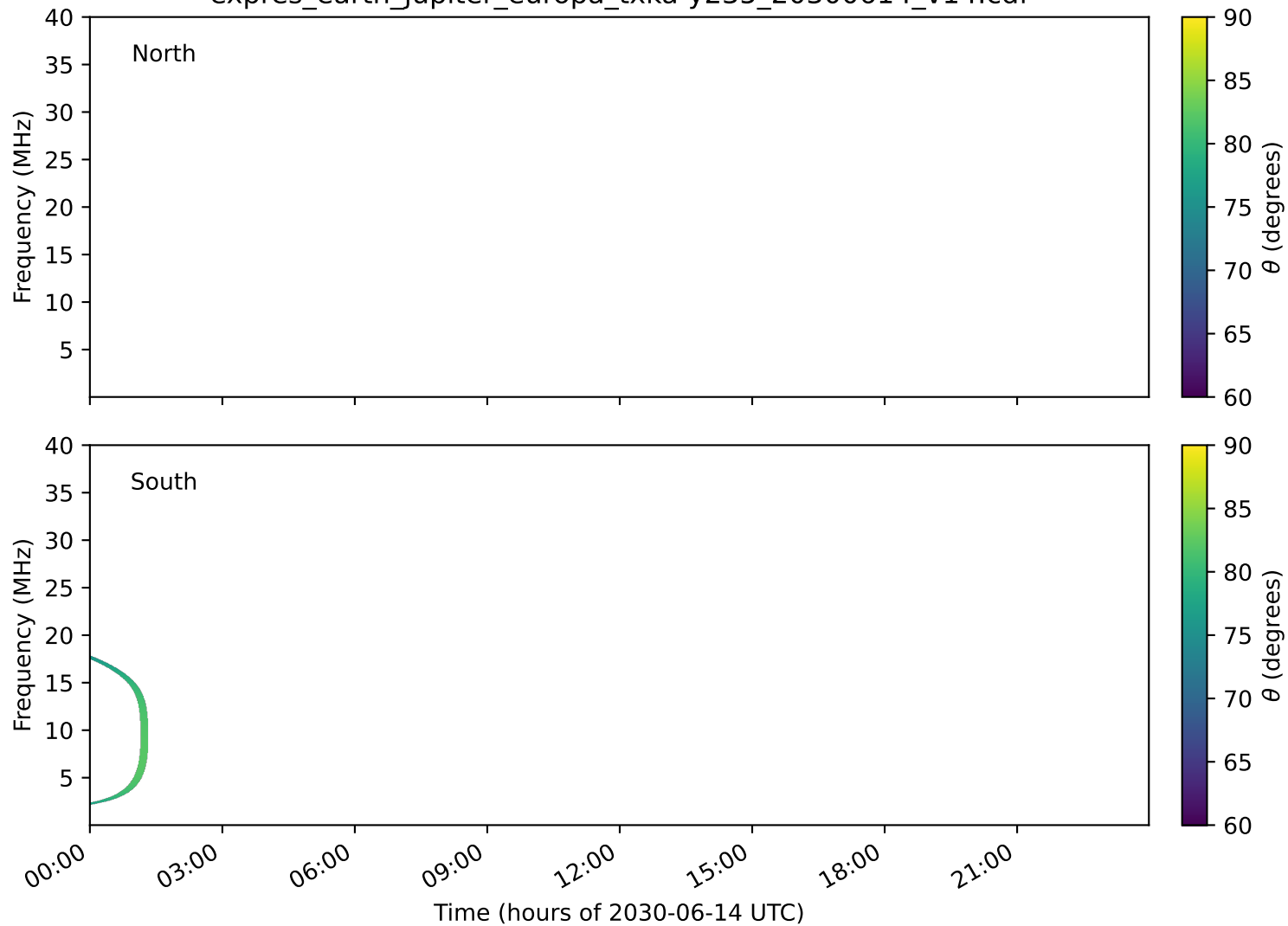
expres_earth_jupiter_europa_txka-y235_20300614_v14.cdf
