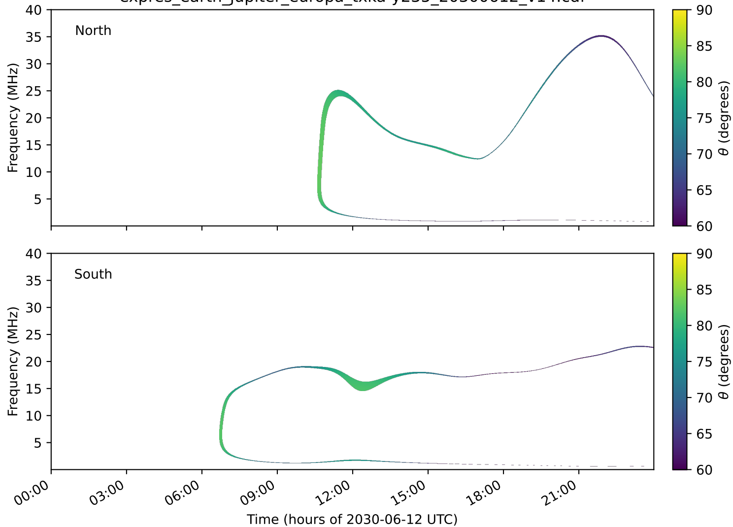
expres_earth_jupiter_europa_txka-y235_20300612_v14.cdf
