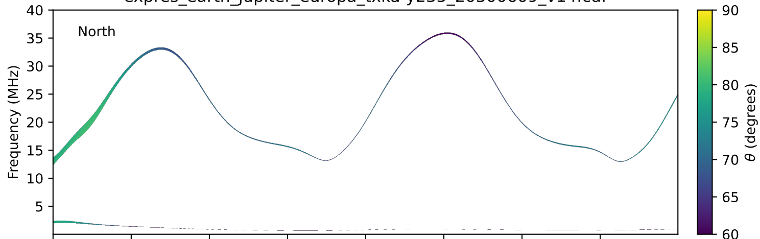
expres_earth_jupiter_europa_txka-y235_20300609_v14.cdf
