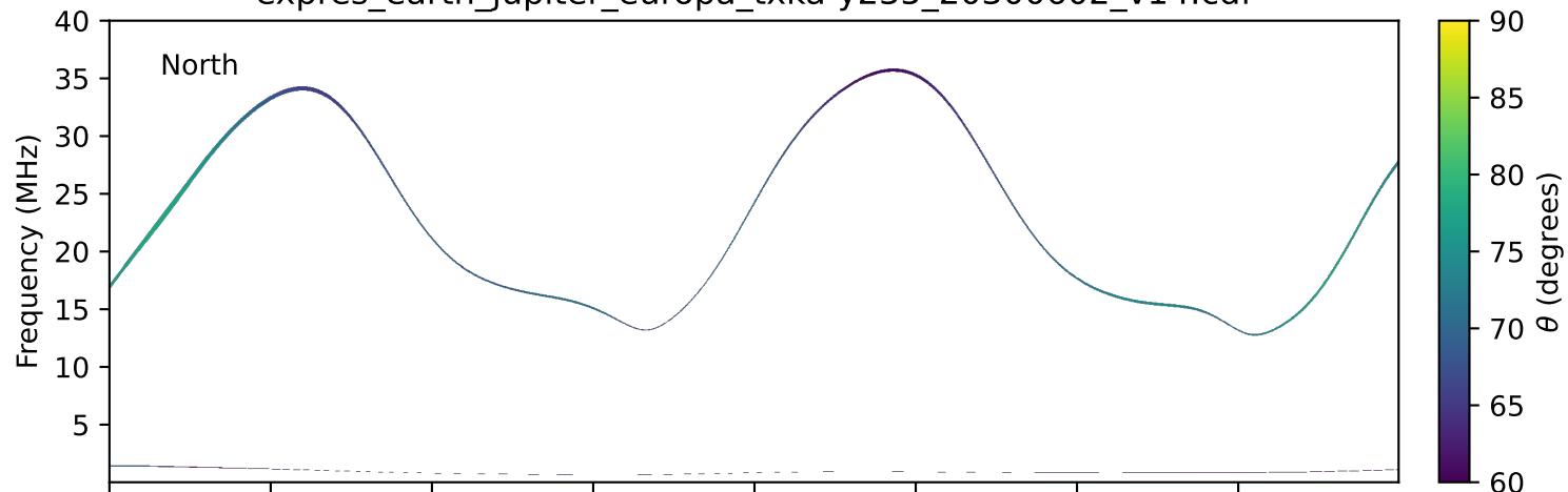
expres_earth_jupiter_europa_txka-y235_20300602_v14.cdf
