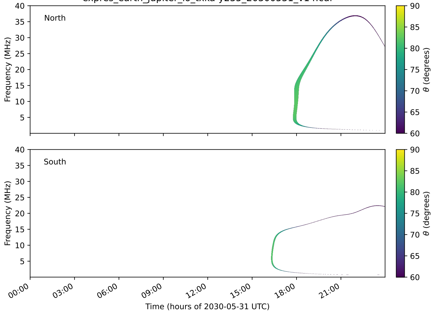
expres_earth_jupiter_io_txka-y235_20300531_v14.cdf
