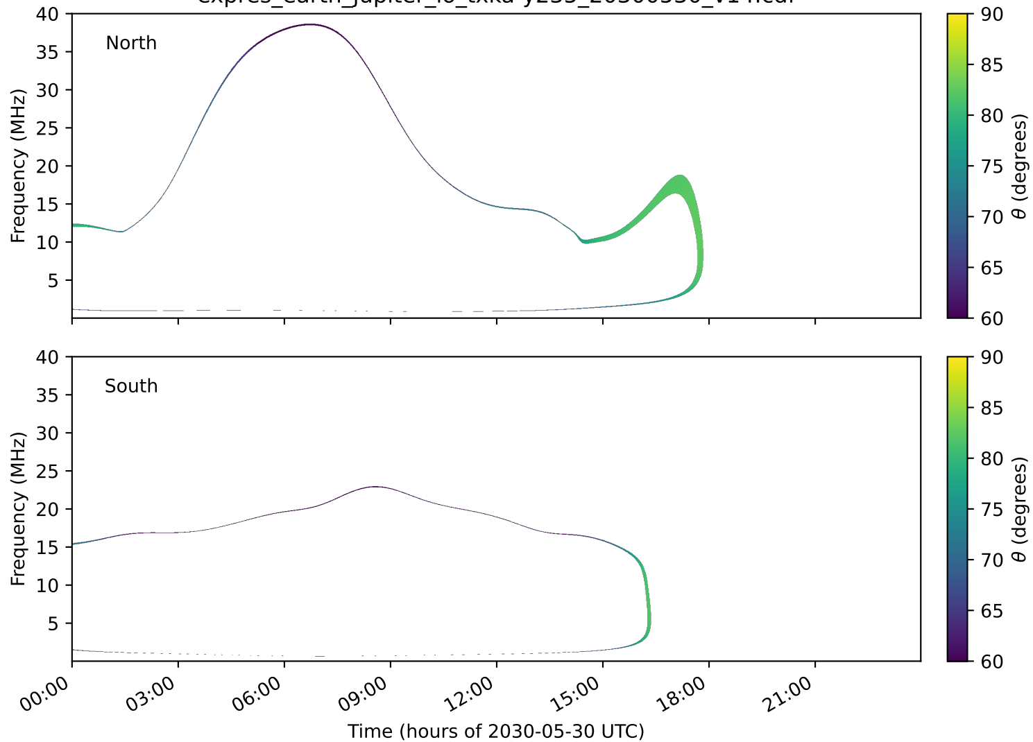
expres_earth_jupiter_io_txka-y235_20300530_v14.cdf
