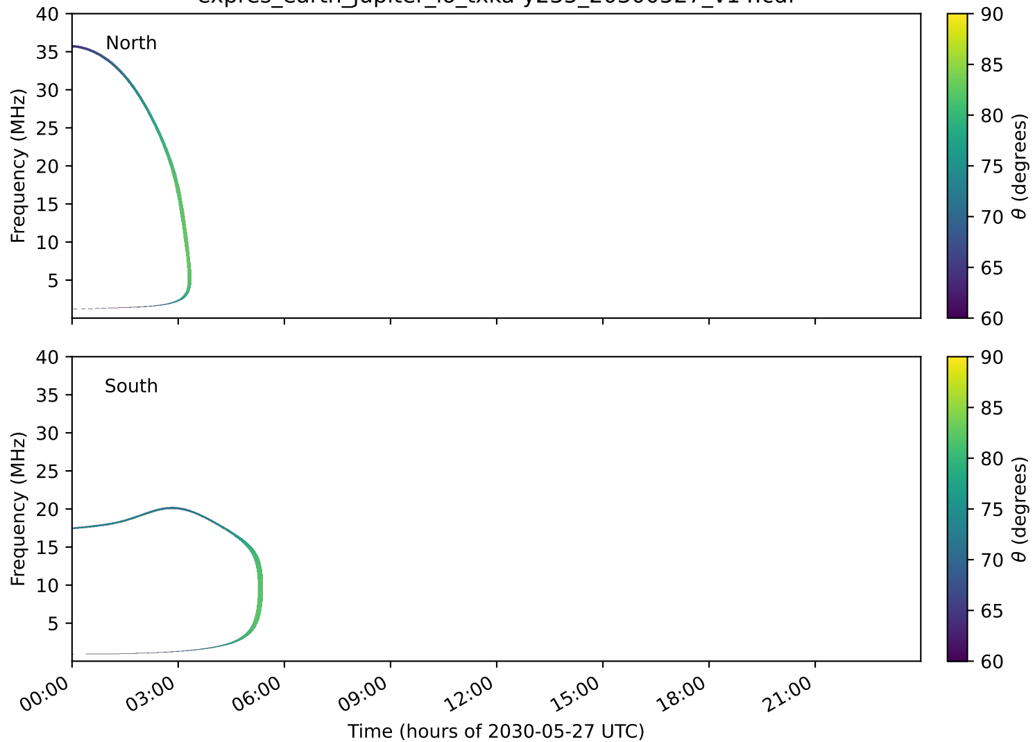
expres_earth_jupiter_io_txka-y235_20300527_v14.cdf
