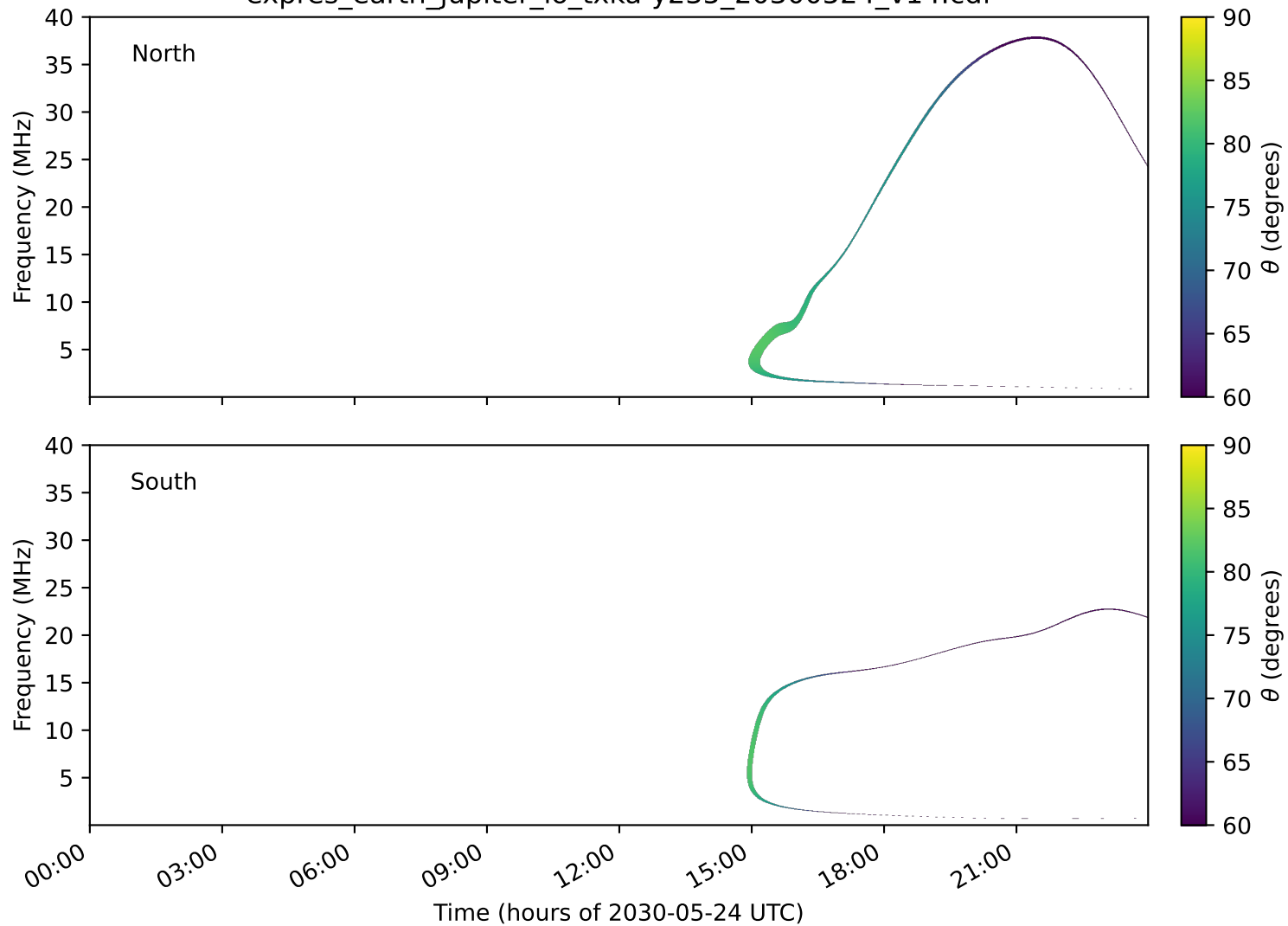
expres_earth_jupiter_io_txka-y235_20300524_v14.cdf
