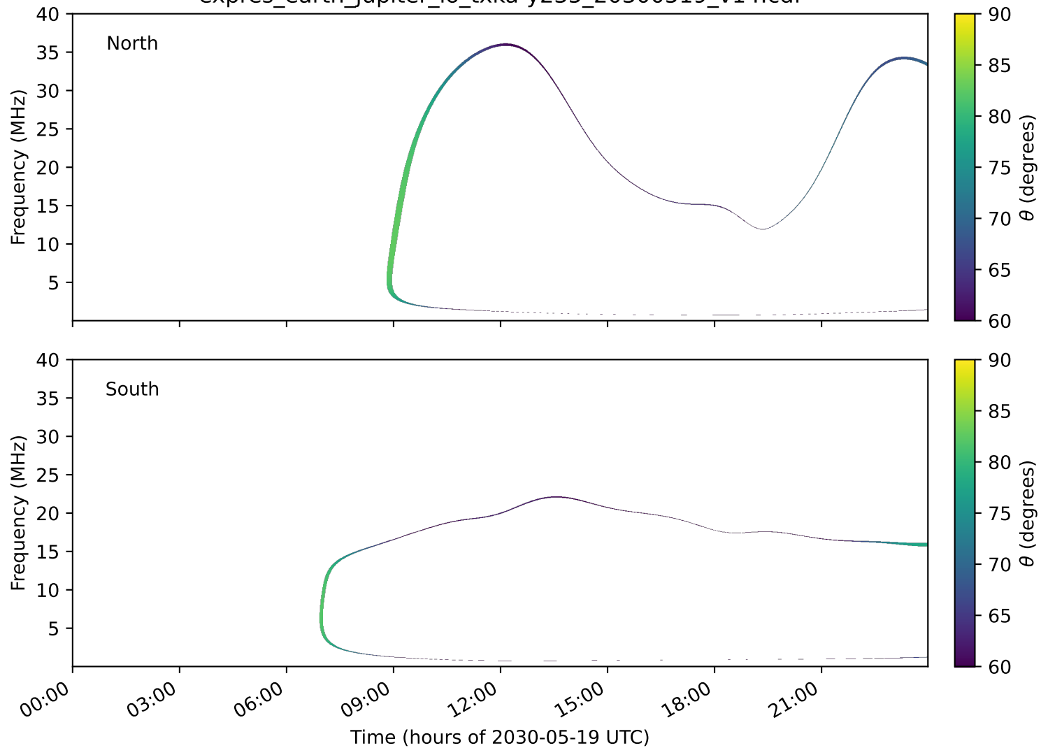
expres_earth_jupiter_io_txka-y235_20300519_v14.cdf
