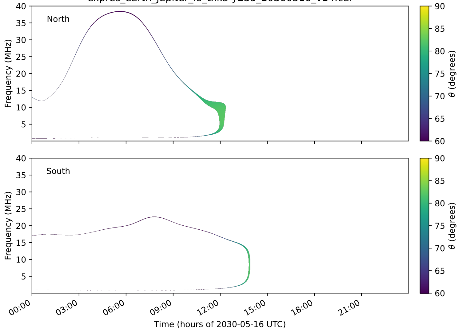
expres_earth_jupiter_io_txka-y235_20300516_v14.cdf
