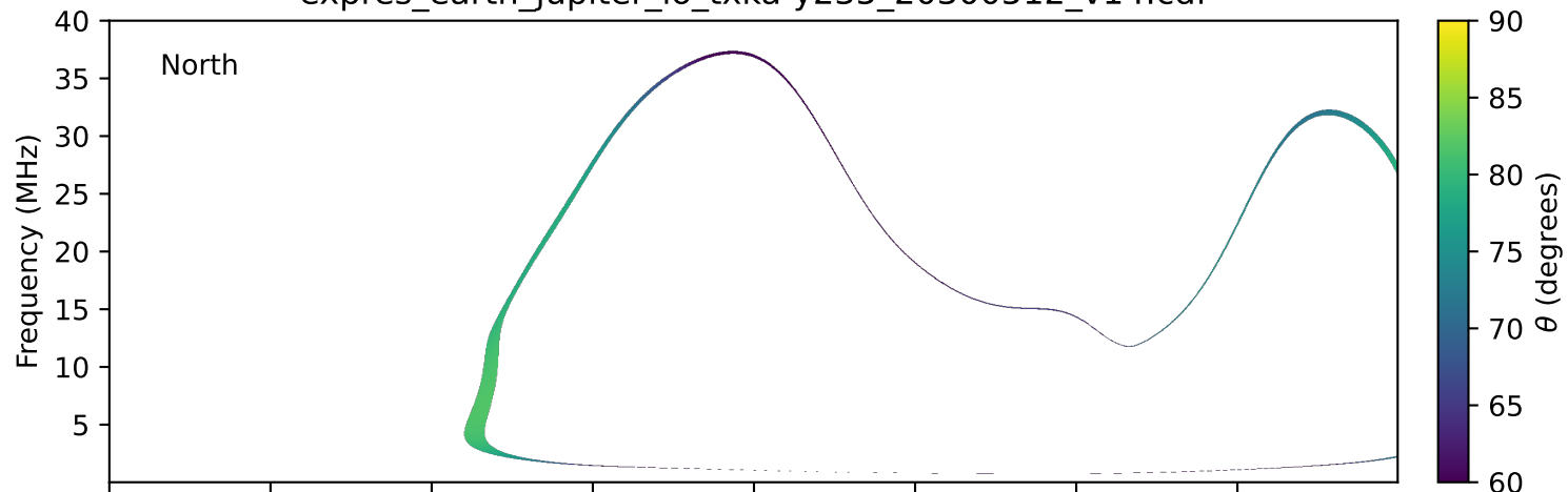
expres_earth_jupiter_io_txka-y235_20300512_v14.cdf
