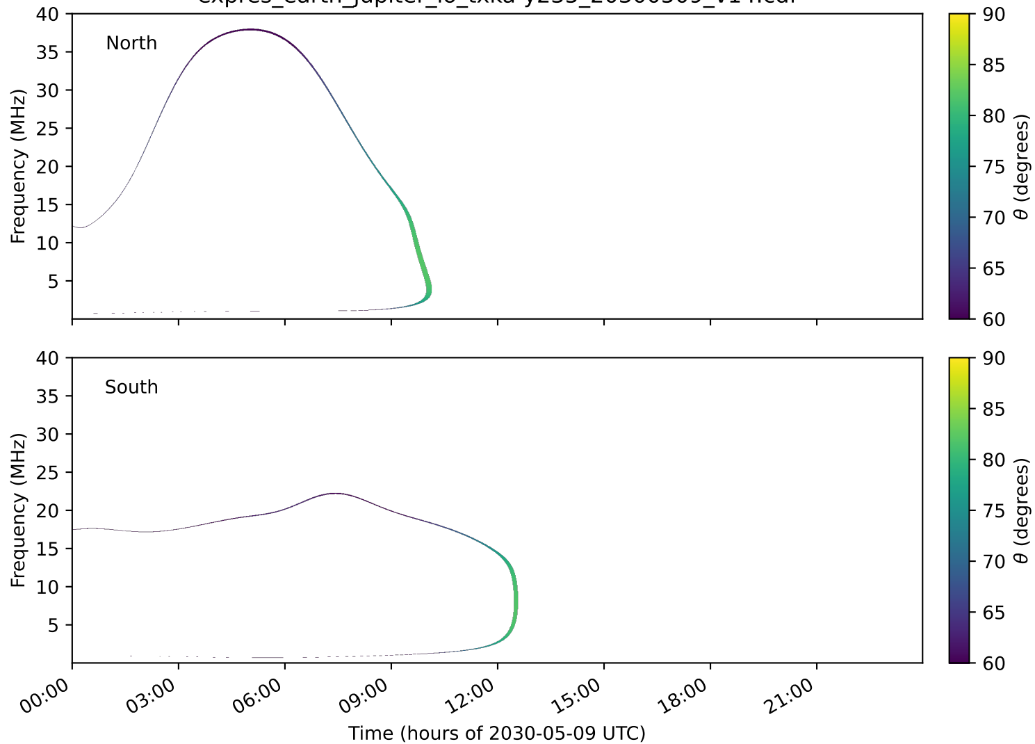
expres_earth_jupiter_io_txka-y235_20300509_v14.cdf
