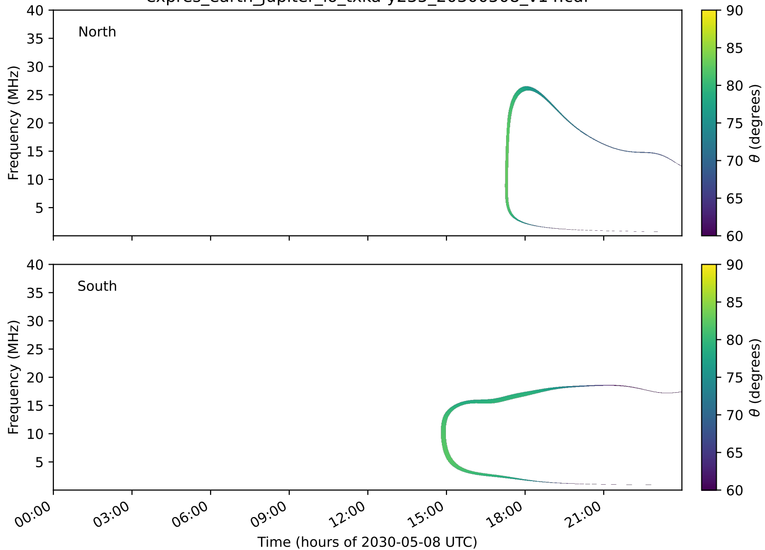
expres_earth_jupiter_io_txka-y235_20300508_v14.cdf
