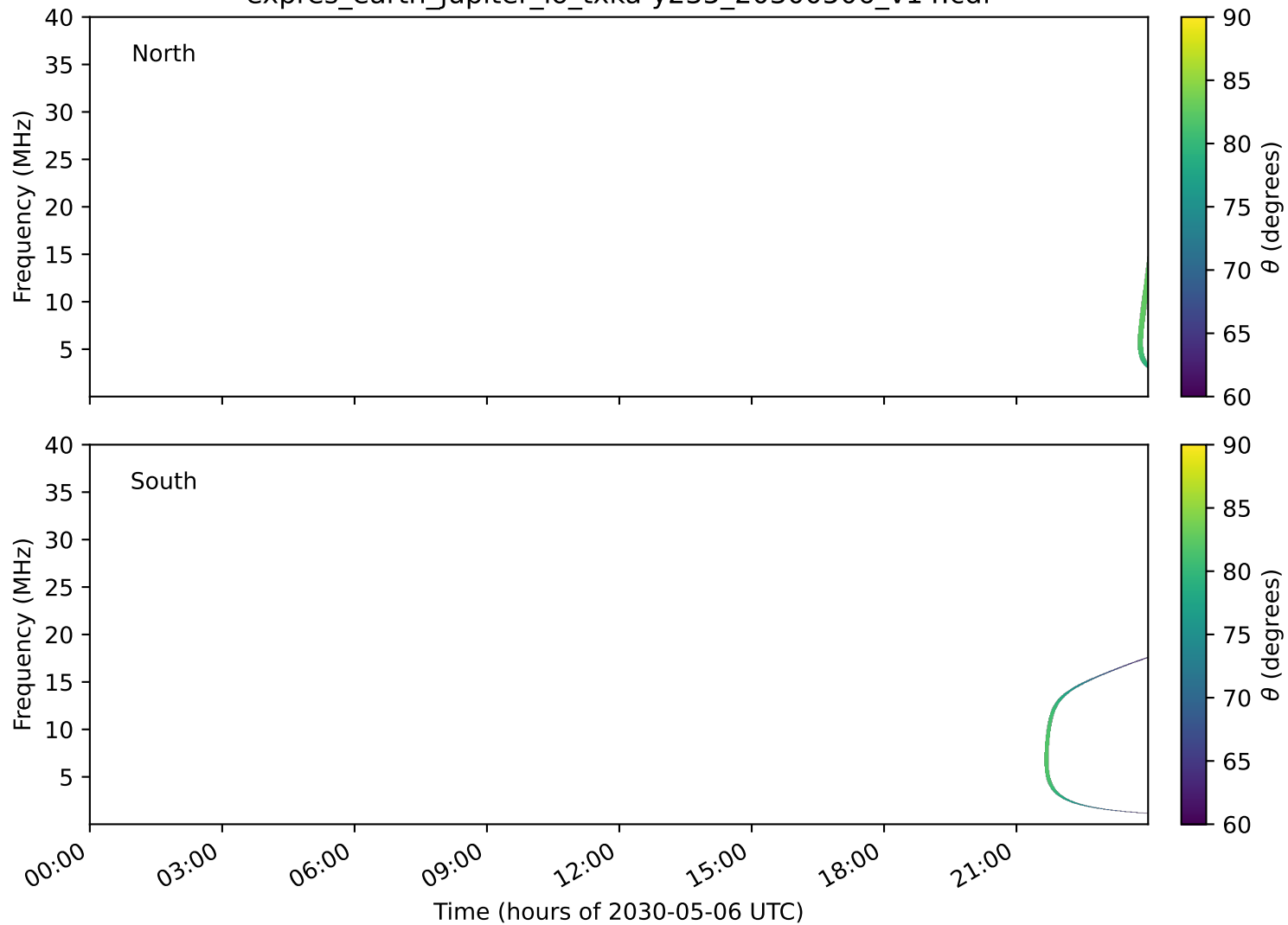
expres_earth_jupiter_io_txka-y235_20300506_v14.cdf
