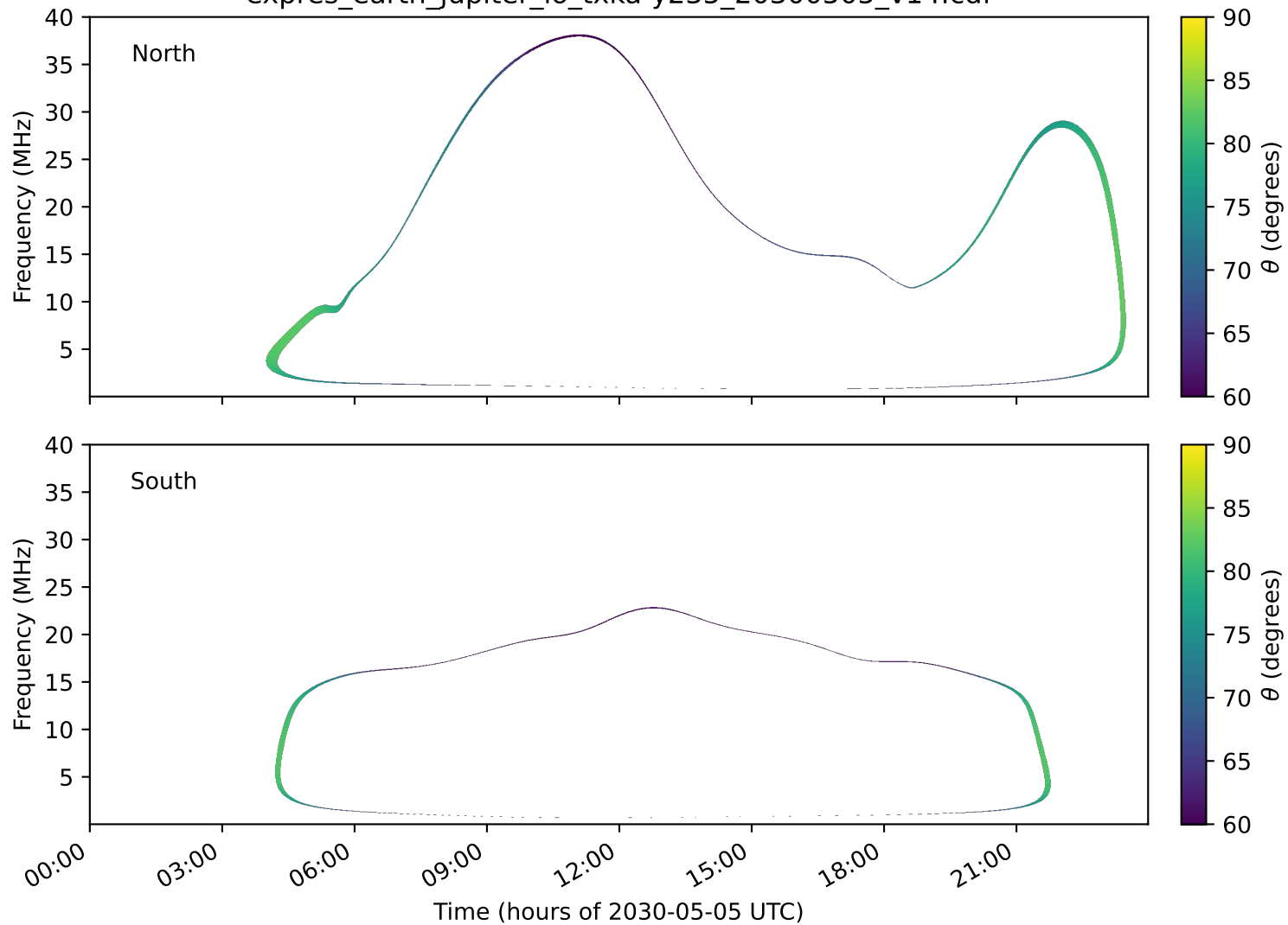
expres_earth_jupiter_io_txka-y235_20300505_v14.cdf
