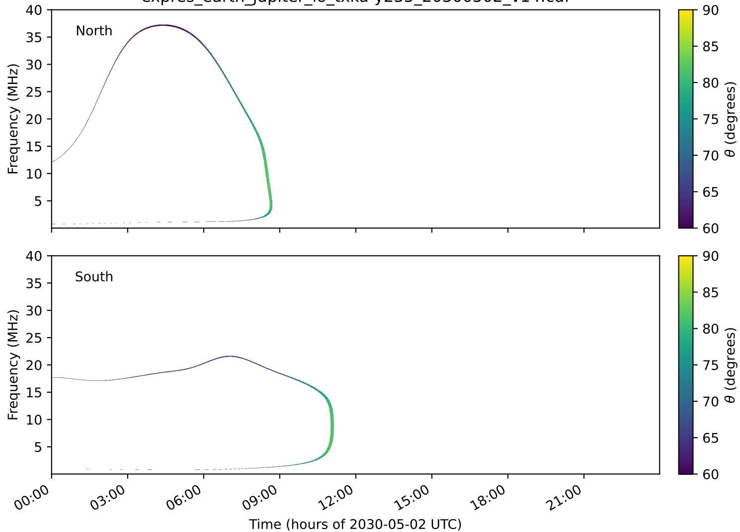
expres_earth_jupiter_io_txka-y235_20300502_v14.cdf
