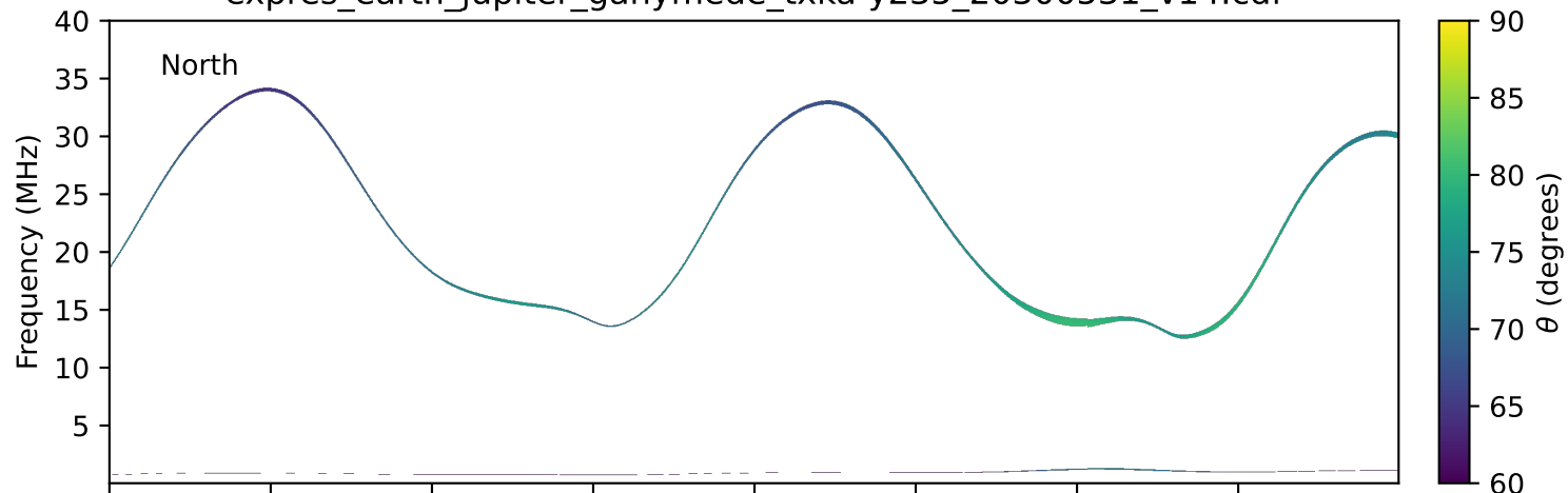
expres_earth_jupiter_ganymede_txka-y235_20300531_v14.cdf
