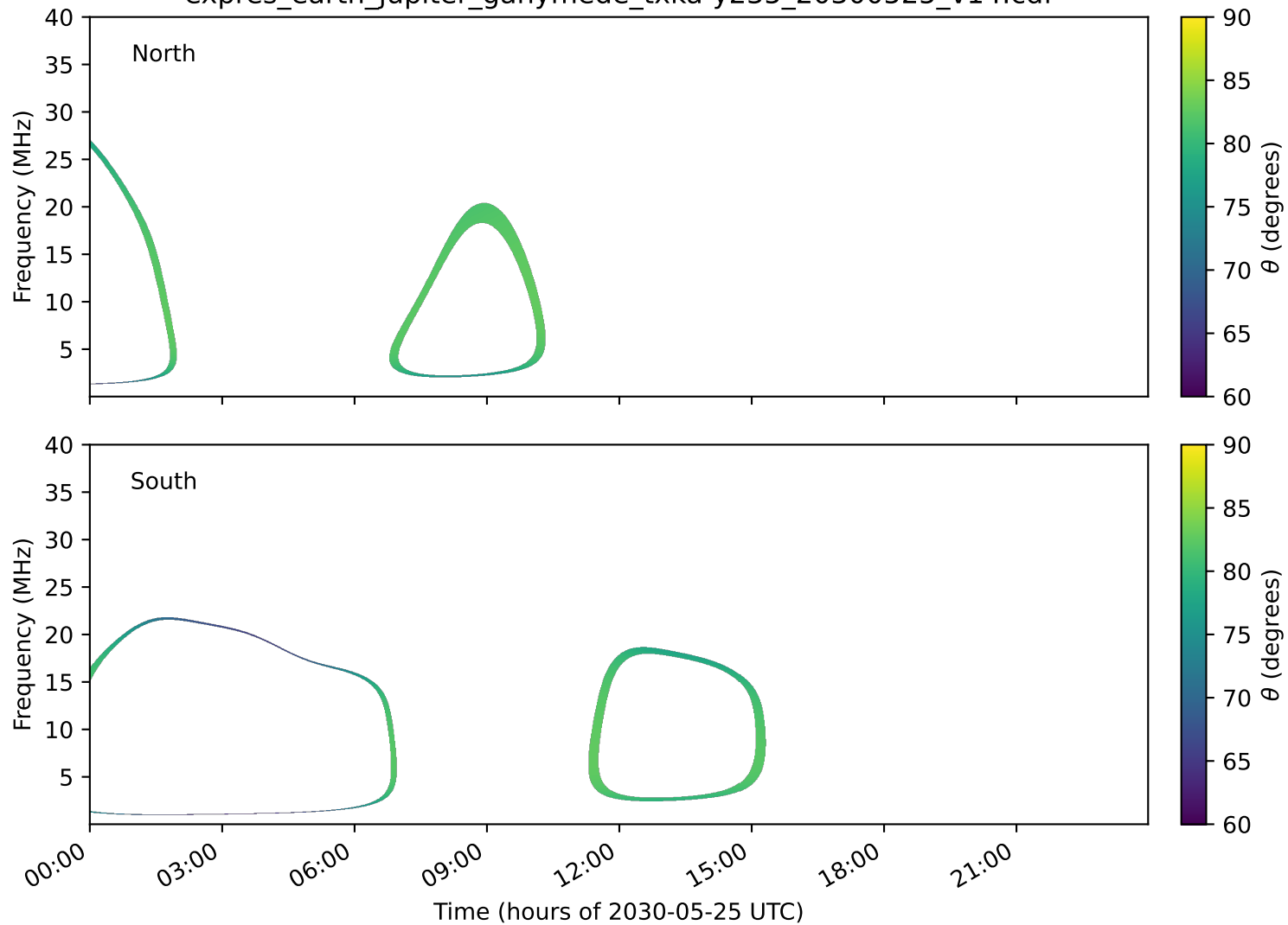
expres_earth_jupiter_ganymede_txka-y235_20300525_v14.cdf
