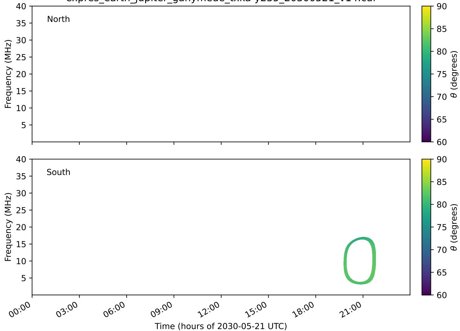
expres_earth_jupiter_ganymede_txka-y235_20300521_v14.cdf
