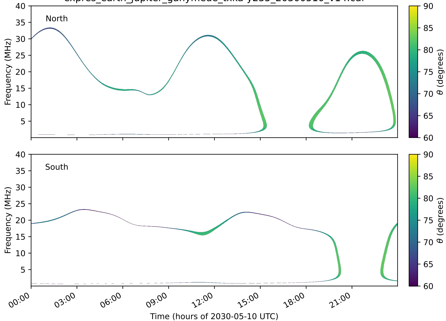
expres_earth_jupiter_ganymede_txka-y235_20300510_v14.cdf
