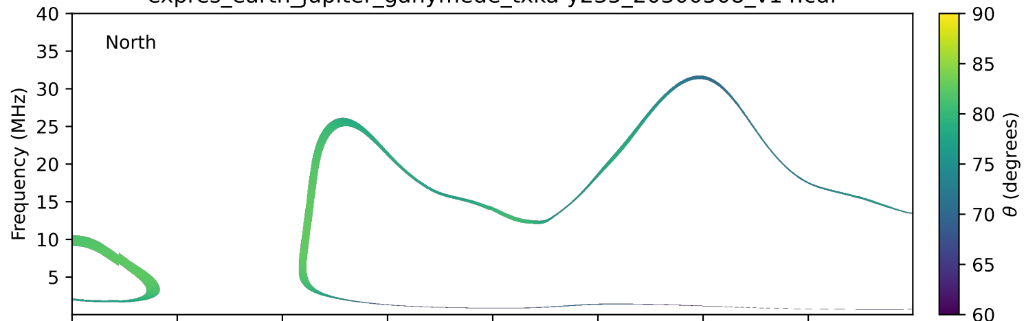
expres_earth_jupiter_ganymede_txka-y235_20300508_v14.cdf
