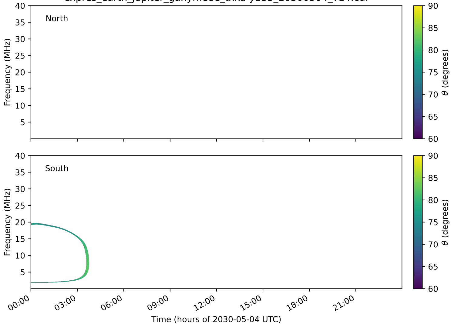
expres_earth_jupiter_ganymede_txka-y235_20300504_v14.cdf
