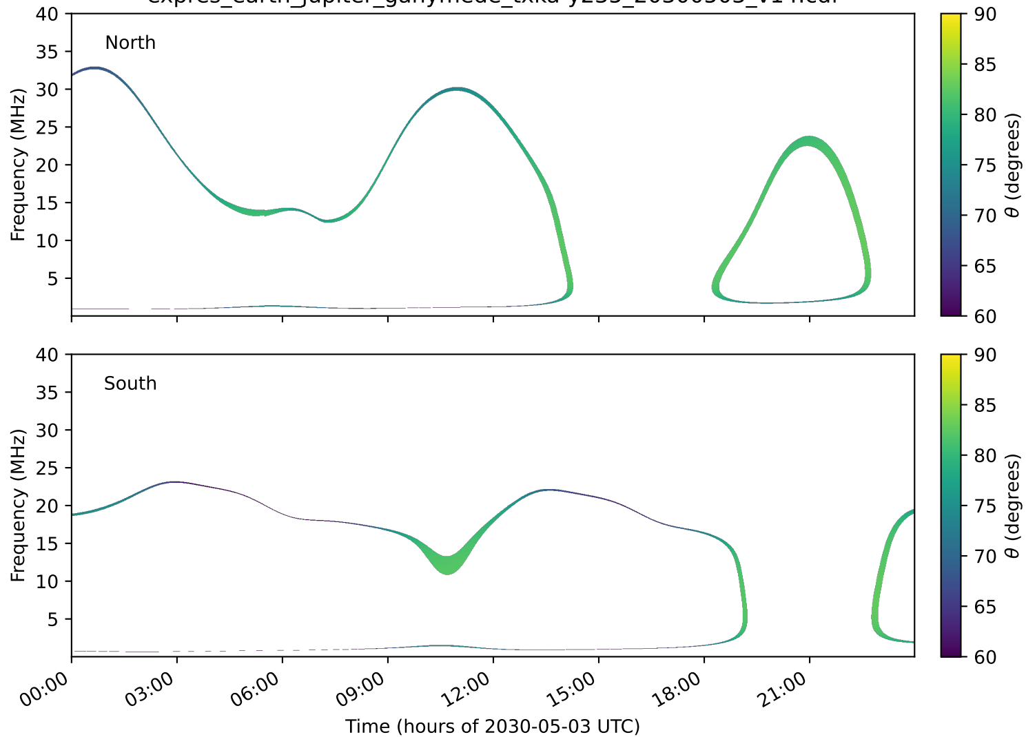
expres_earth_jupiter_ganymede_txka-y235_20300503_v14.cdf
