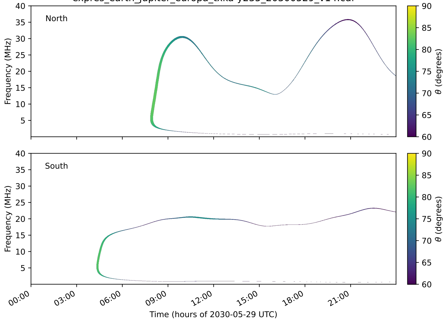
expres_earth_jupiter_europa_txka-y235_20300529_v14.cdf
