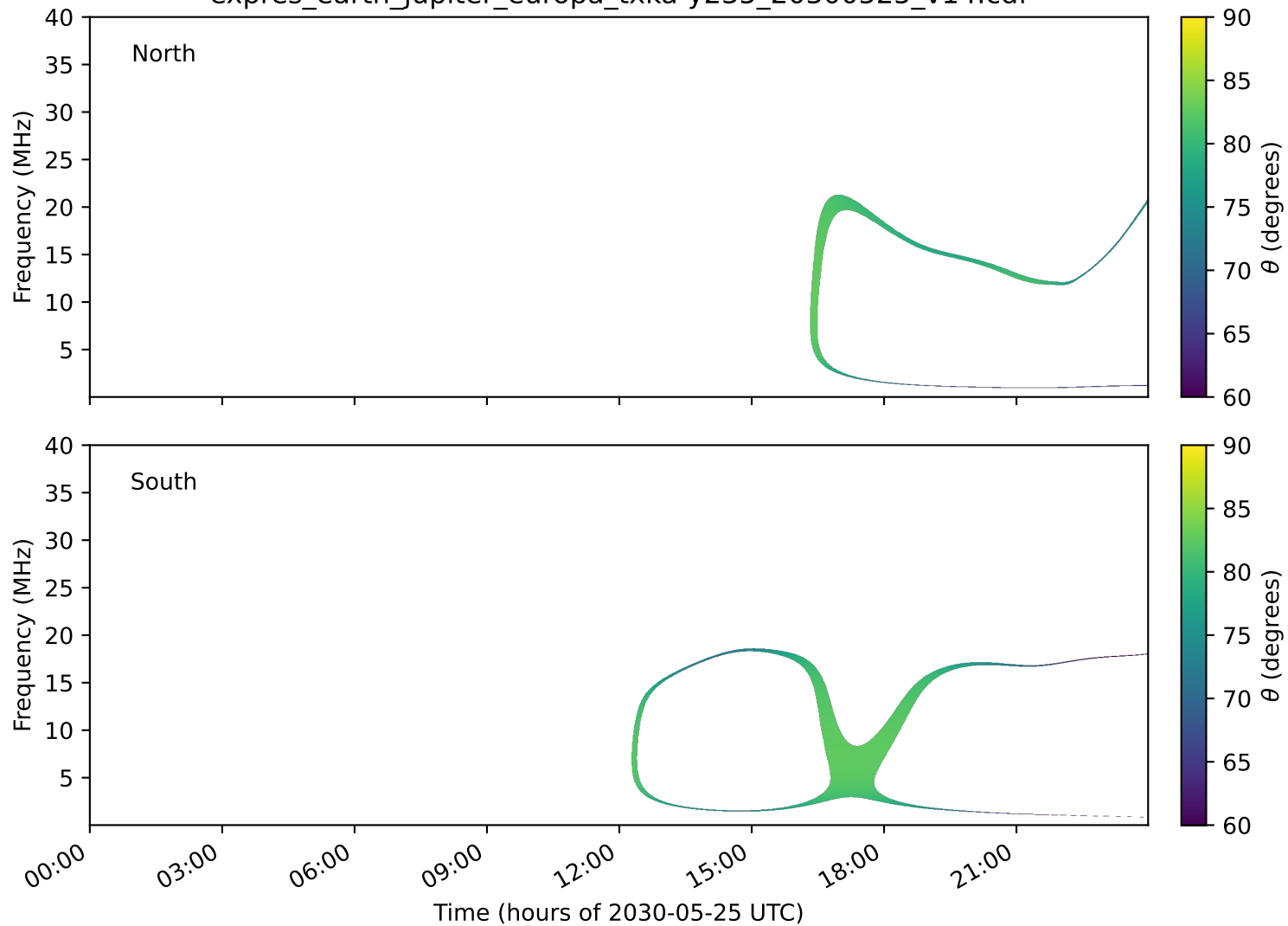
expres_earth_jupiter_europa_txka-y235_20300525_v14.cdf
