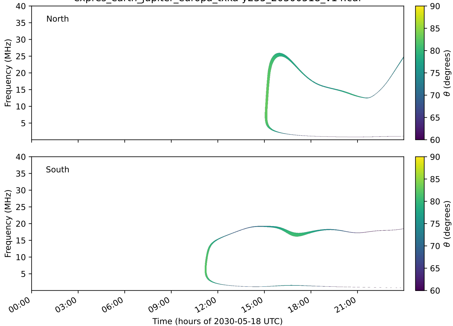
expres_earth_jupiter_europa_txka-y235_20300518_v14.cdf
